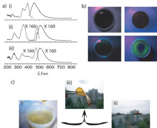
Figure 3. Evolution of the optical properties of the metallodynamers: a) Excitation (dashed line) and emission (solid line) spectra of: i) P2 , ii) P3 , and iii) polymer blend B2 in \text{CHCl}_3 (0.2 mm). b) Photographs of the metallodynamer films taken under excitation at 365 nm: nonfluorescent films P2 (top left), P4 (top right), B2 before the exchange reaction (bottom left); fluorescent film B2 after exchange (bottom right). c) Evolution of the mechanical properties of the metallodynamers: i) P2 (gum), ii) P4 (hard film), and iii) blend B2 (soft film).
